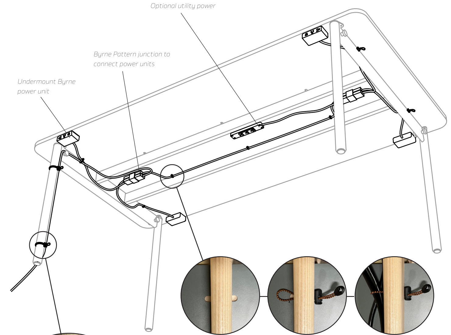
There are slots routed between the surface and the wood frame.
